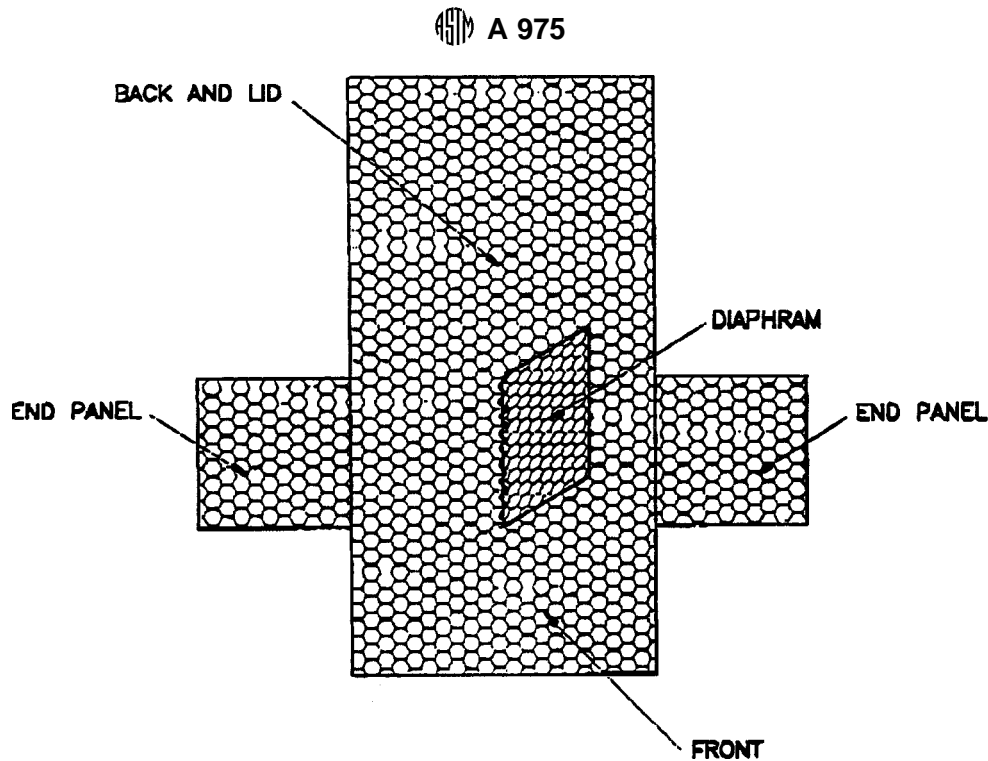
FIG. 2 Mechanically Manufactured Gabion
